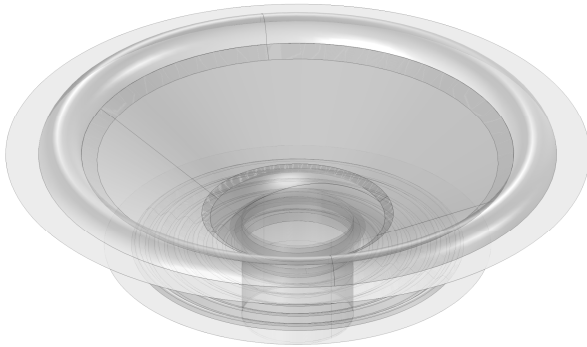
Figure 6 3D surface based CAD model of vibration system
